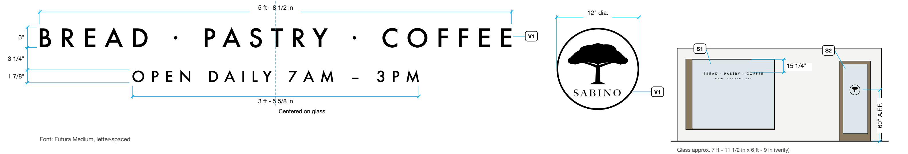
B.1 Window Vinyl – Copy Layout Scale: 1 1/2" = 1'-0"
