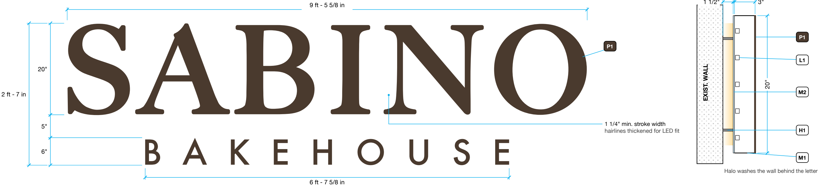
A.1 Halo-Lit Channel Letters – Dimensions Scale: 1" = 1'-0"
